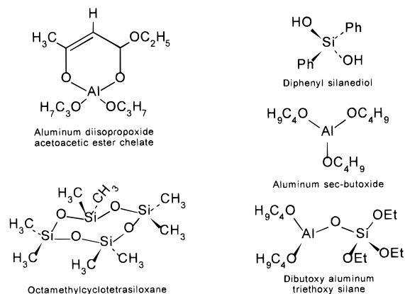
Figure 1. Monomeric schematics of the chemicals used in this study.
